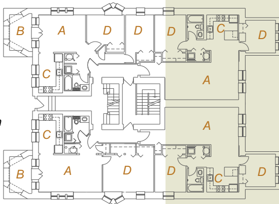
floor plan
